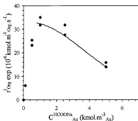
Figure 4. Influence of the sodium formate concentration on the observed initial reaction rate r_{Org}^i ( C_{Org}^{DMI} = 0.1 \text{ kmol.m}^{-3}_{Org} , C_{Aq}^{Rh} = 0.002 \text{ kmol.m}^{-3}_{Aq} , \alpha = 1 , TPPTS/Rh = 6); the points represent the experimental data and the curves represent the semi-empirical model described by Equation 5
