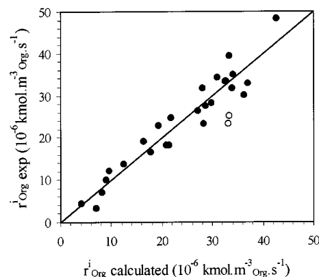
Figure 6. Calculated vs. experimental initial rates of reaction; con- ductions see Table 2 except for symbol ( \circ ) for which C_{Aq}^{HCOONa} = 0.5 \text{ kmol.m}^{-3}_{Aq}
