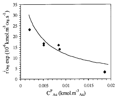
Figure 3. Influence of the phosphane concentration on the observed initial reaction rate r_{Org}^i ( C_{Org}^{DMI} = 0.1 \text{ kmol.m}^{-3}_{Org} , C_{Aq}^{Rh} = 0.002 \text{ kmol.m}^{-3}_{Aq} , \alpha = 1 , C_{Aq}^{HCOONa} = 5 \text{ kmol.m}^{-3}_{Aq} ); the points represent the experimental data and the curves represent the semi-empirical model described by Equation 5
