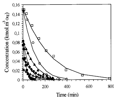
Figure 5. Concentration vs. time profiles. Comparison between experimental data (symbols) and semi-empirical model (lines). ( \Delta ): Standard test: T = 313 \text{ K} ; C_{Org}^{DMI} = 0.1 ; C_{Aq}^{HCOONa} = 5 , TPPTS/Rh = 6.3, \alpha = 1 , C_{Aq}^{Rh} = 0.002 . Other tests: same with: ( \circ ) \alpha = 0.2 ; ( \blacklozenge ): \alpha = 0.53 , C_{Aq}^{Rh} = 0.005 ; ( \square ): C_{Org}^{DMI}(0) = 0.155 , C_{Aq}^{HCOONa} = 1 ; ( \blacksquare ): C_{Org}^{DMI}(0) = 0.05 , C_{Aq}^{HCOONa} = 2.5 ; ( \bullet ): TPPTS/Rh = 3.1. Units: C_{Org}^{DMI} in \text{kmol.m}^{-3}_{Org} ; C_{Aq}^{HCOONa} and C_{Aq}^{Rh} in \text{kmol.m}^{-3}_{Aq} ; \alpha in \text{m}^3_{Org} \cdot \text{m}^{-3}_{Aq} .
