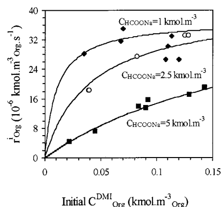
Figure 2. Influence of the initial substrate concentration on the observed initial reaction rate r_{\text{Org}}^i for different sodium formate concentrations ( C_{\text{Aq}}^{\text{Rh}} = 0.002 \text{ kmol}\cdot\text{m}^{-3}_{\text{Aq}} , \alpha = 1 , TPPTS/Rh = 6, 313 K); the points represent the experimental data and the curves represent the semi-empirical model described by Equation 5
