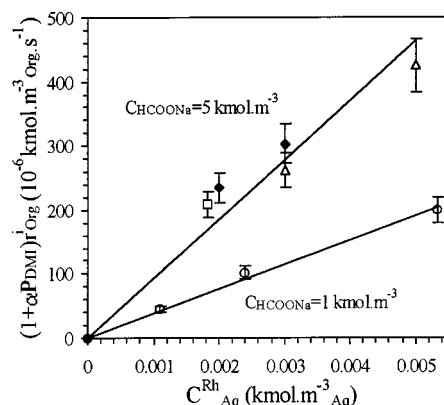
Figure 1. Influence of the catalyst concentration on the observed initial reaction rate r_{\text{Org}}^i [ T = 313 \text{ K} , C_{\text{Org}}^{\text{DMI}} = 0.155 \text{ kmol}\cdot\text{m}^{-3}_{\text{Org}} , TPPTS/Rh = 6; (♦ and ○): \alpha = 1 ; (Δ): \alpha = 0.5 ; (□): \alpha = 0.45 ]
