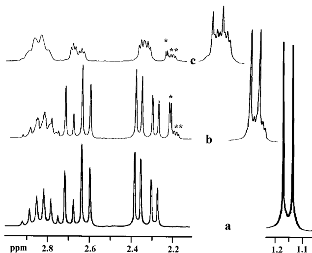
Figure 7. ^1\text{H} -NMR spectra of DMS (a) and of the products from reduction in \text{DCOONa}/\text{H}_2\text{O} (b) and in \text{HCOONa}/\text{D}_2\text{O} (c); signals of the vinylic proton in the by-product DMM: (*) 5, (**) 6 (see Table 5)
